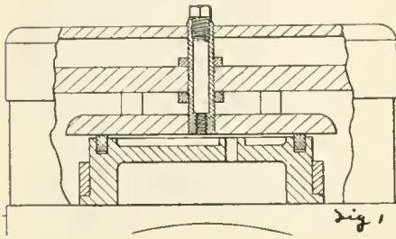
VALVE WITH TEST PLUG.
